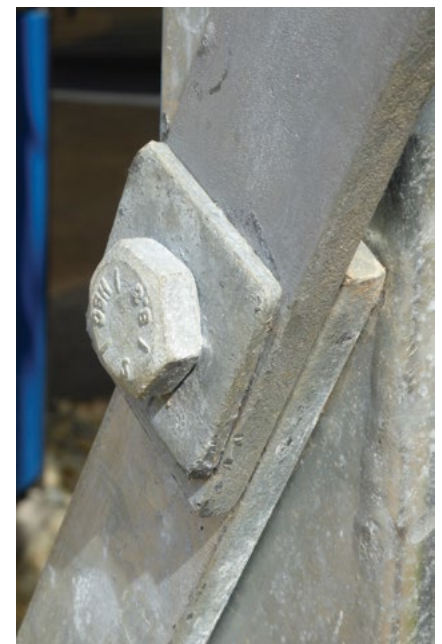
Figure 16: High strength bolted connection joining multiple plies
