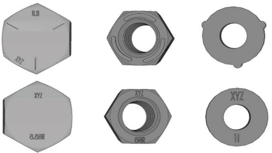
Figure 11: Marking for class 8.8 high strength bolts, nuts and washers
