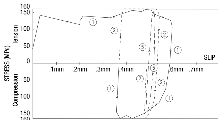
Figure 24: Cyclic stress v slip for fatigue samples with hot dip galvanized plates and bolts
