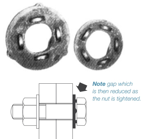
Figure 21: Load indicating washers fitted under bolt head
