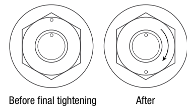
Figure 20: Part turn tightening showing location marks in the before and after positions
